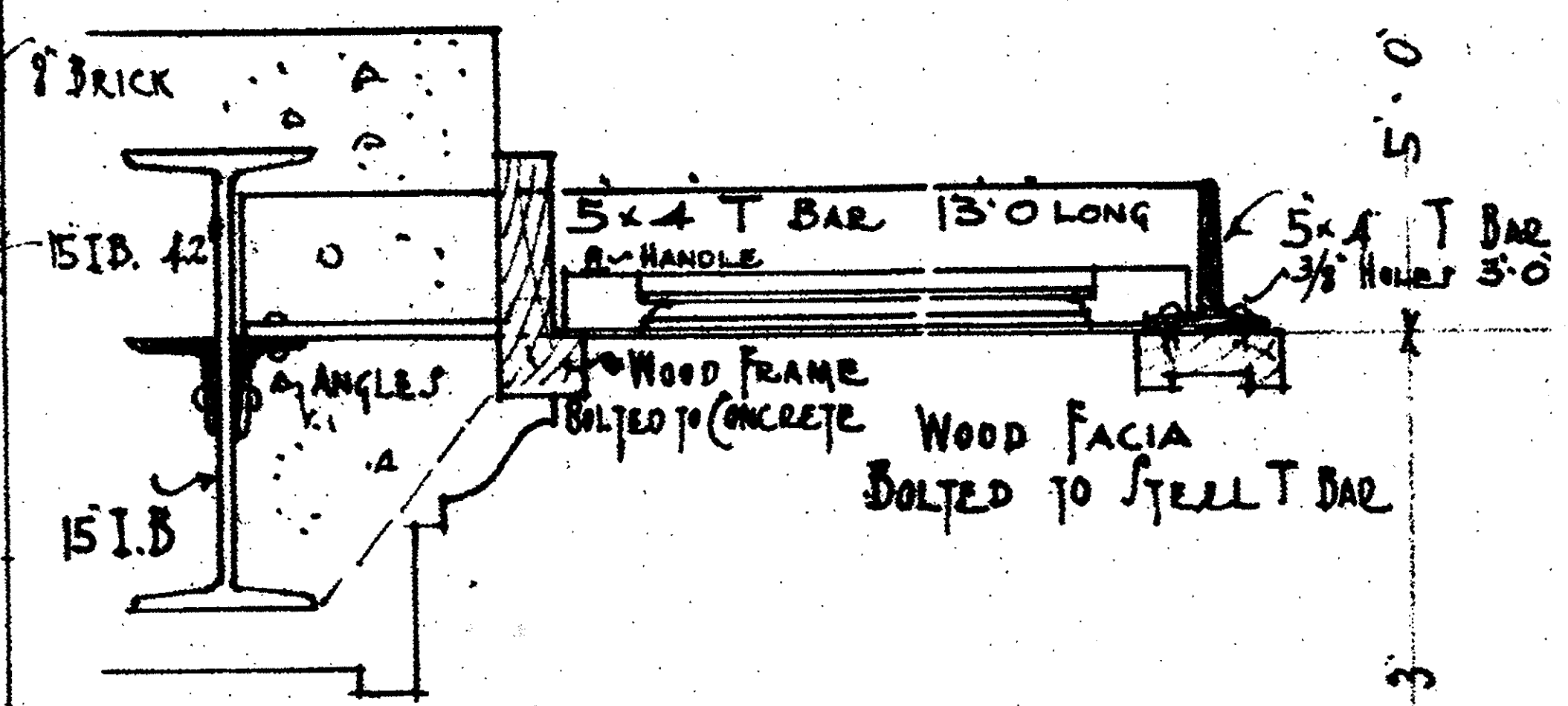
DETAIL SKYLIGHT CONSTRUCTION
